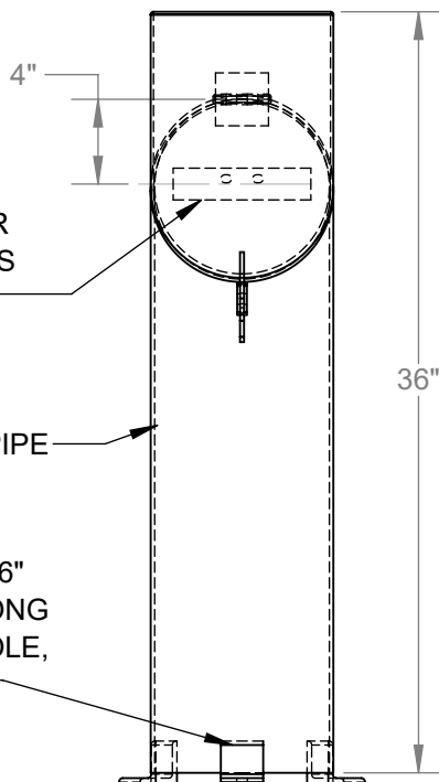
FRONT
